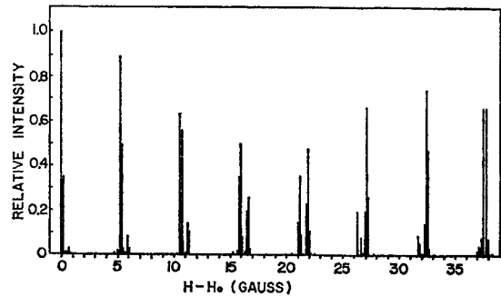
FIG. 3. Hyperfine lines predicted for the F -center ESR absorption spectrum in \text{Li}^6\text{F} . The central line and first 84 lines on the high-field side of the spectrum are shown.
