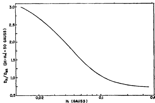
FIG. 9. Reconstruction of the ESR spectrum of sample No. 3a, according to the exchange-narrowing model. The ratio of the derivative intensity of the normal F -center component, D_n|H-H_0| , to that of the exchange narrowed component, D_{en}|H-H_0| , is shown as a function of H_1 .
