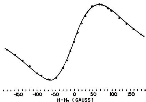
FIG. 12. Reconstruction of the ESR spectrum of sample No. 3a. The theoretical composite line shape, indicated by the circles, is compared at a low microwave power level with the observed resonance, represented by the solid line.
