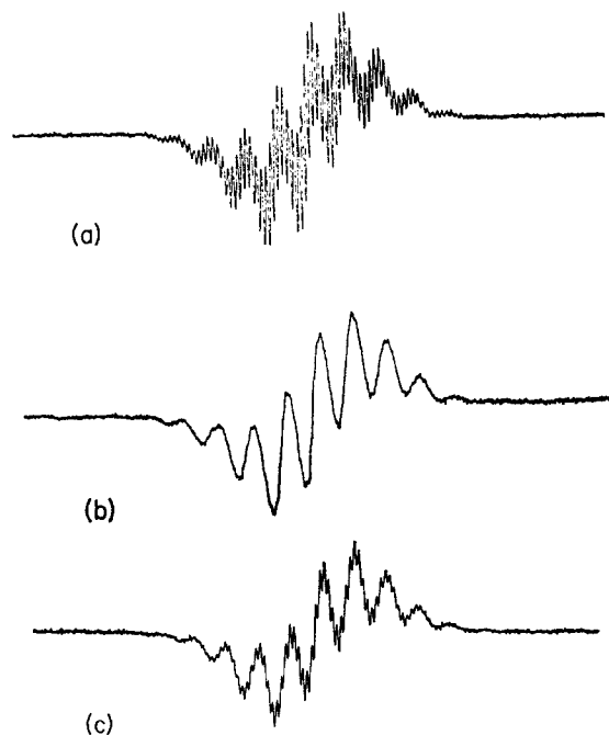
FIG. 5. ESR spectra observed for neutron-irradiated single crystals of \text{LiF} . (a) \text{Li}^6\text{F} , \mathbf{H} along [111] . (b) \text{Li}^6\text{F} , \mathbf{H} along [100] . (c) \text{Li}^6\text{F} , \mathbf{H} along [110] . Scan rates in all traces are equal and are the same as that of the trace of Fig. 1.
