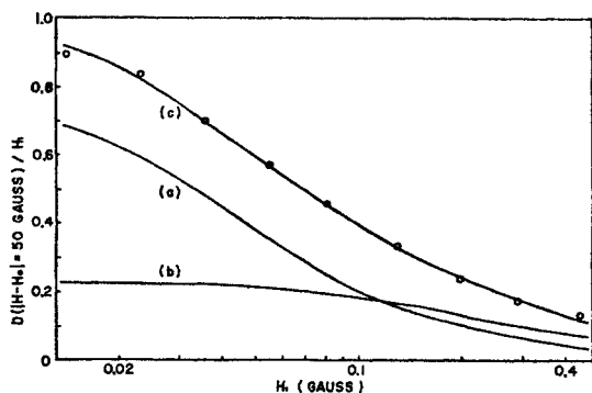
FIG. 10. Reconstruction of the ESR spectrum of sample No. 3a. (a) Saturation of the normal F -center component alone. (b) Saturation of the exchange-narrowed component alone. (c) Variation of the sum of curves (a) and (b) with H_1 . The data points show the observed dependence of derivative intensity on H_1 .
