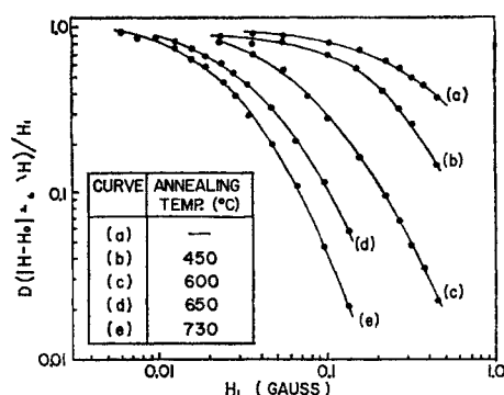
FIG. 14. Saturation of the ESR spectrum of sample No. 9 as a function of the temperature at which the sample was annealed.
