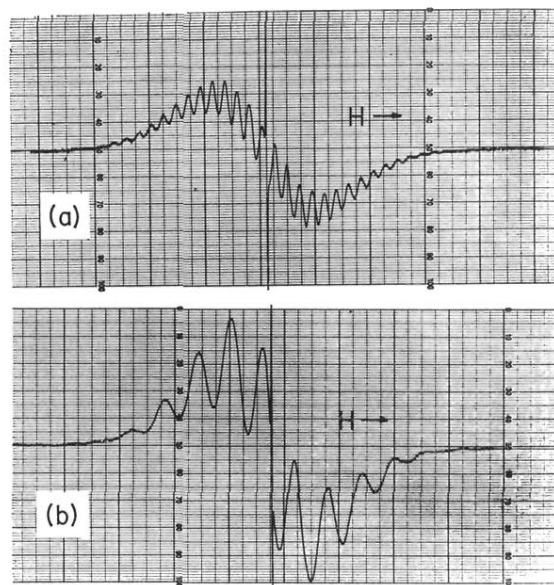
FIG. 2. Recorder traces similar to those used for evaluating the g shift of the F -center spectrum in normal LiF, (a), and Li 6 F, (b). The sharp central line is due to conduction electrons in small particles of lithium metal observed simultaneously with the LiF crystals. The direction of increasing magnetic field scan is indicated by the arrows. The applied field \mathbf{H} is along [111] in (a), and [100] in (b).
