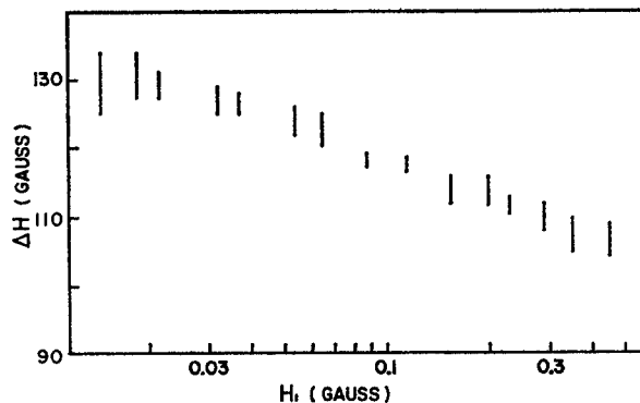
FIG. 7. Dependence of envelope width \Delta H on the microwave magnetic field amplitude H_1 , for sample No. 1.
