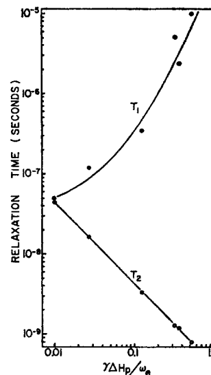
FIG. 13. Variation of T_1 and T_2 with \gamma\Delta H_p/\omega_e for six LiF samples, according to the exchange-narrowing model. The value of T_1 at \gamma\Delta H_p/\omega_e=0.125 is an upper limit for sample No. 6a, as explained in the text. The order of the samples represented by the data points is as follows, from right to left along the horizontal axis: 3a, 4a, 5a, 6a, 7b, 8a.
