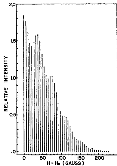
FIG. 4. Construction of the F -center hyperfine absorption spectrum that should be observable in \text{Li}^6\text{F} when \mathbf{H} is along [111] .
