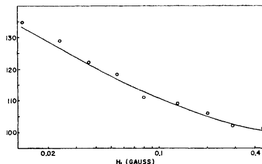
FIG. 11. Reconstruction of the ESR spectrum of sample No. 3a. The solid curve shows the dependence of the width of the theoretical composite resonance on H_1 . The observed dependence on H_1 is given by the data points.
