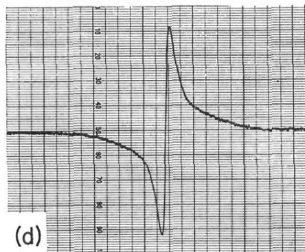
FIG. 8. Variation of ESR spectra of neutron-irradiated LiF with neutron dose. (a) Sample No. 3a, 10^{16}n/cm^2 , H intermediate between [100] and [110]. (b) Sample No. 4a, 10^{17}n/cm^2 , H intermediate. (c) Sample No. 5a, 10^{18}n/cm^2 , H along [110]. (d) Sample No. 6a, 5 \times 10^{18}n/cm^2 , H intermediate. (e) Sample No. 7a, 5 \times 10^{18}n/cm^2 , H along [111]. (f) Sample No. 7b, 5 \times 10^{18}n/cm^2 , H along [111].
