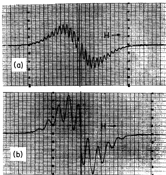
FIG. 2. Recorder traces similar to those used for evaluating the g shift of the F -center spectrum in normal LiF, (a), and \text{Li}^6\text{F} , (b). The sharp central line is due to conduction electrons in small particles of lithium metal observed simultaneously with the LiF crystals. The direction of increasing magnetic field scan is indicated by the arrows. The applied field \mathbf{H} is along [111] in (a), and [100] in (b).
