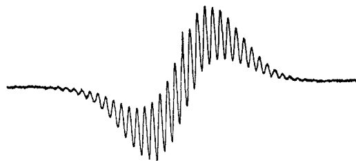
FIG. 1. ESR spectrum of a neutron-irradiated crystal of normal LiF with H along [111] . The neutron dose was 10^{16} n/cm 2 .
